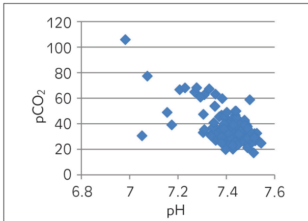
Figure 1 pH vs p\text{CO}_2 .
