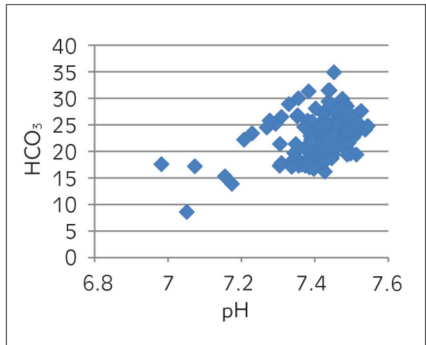
Figure 4 pH vs \text{HCO}_3 .
