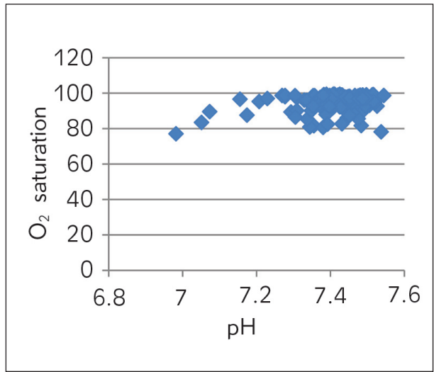
Figure 3 pH vs \text{O}_2 saturation.
